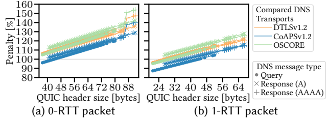
Fig. 9. Relative amount of additional link layer data required by DNS over QUIC compared to other DNS transports when resolving a name with a length of 24 characters for a single record (A or AAAA).
