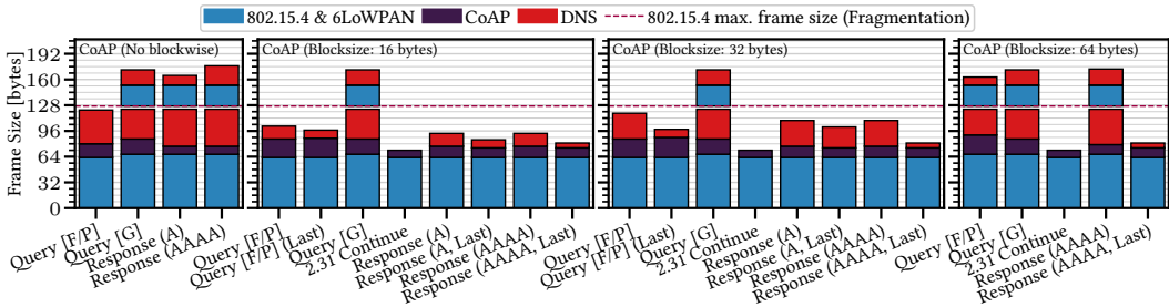
Fig. 14. Maximum link layer packet sizes for each transport when resolving a name with a length of 24 characters for a single record (A and AAAA respectively) for different CoAP methods (F = FETCH, G = GET, P = POST) and block sizes. “Last” denotes the size of the last block with block-wise transfer.
