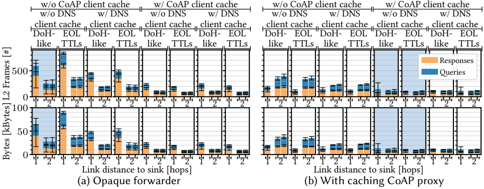
Fig. 10. Link utilization for four AAAA record queries (Poisson-distributed with \lambda = 5 queries / s) for different caching solutions with CoAP FETCH, comparing DoH-like and EOL TTLs caching approaches. The scenarios highlighted in blue are evaluated in detail in Section 6.3.
