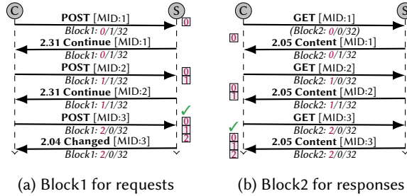
Fig. 12. Different block-wise transfers of a 96 bytes body between a client C and a server S using 32 byte blocks in CoAP. n/m/s denotes the block number, whether more blocks (or not) can be sent, and the block size.
