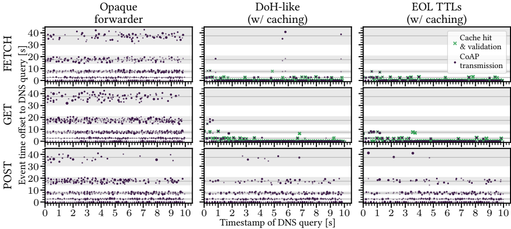
Fig. 11. CoAP events of message (re-)transmissions at the client compared to the time of the initial DNS query. Retransmissions follow an exponential back-off and scatter within specific (gray) areas. Size and opacity of each marker represent the multiplicity of events in the same area.
