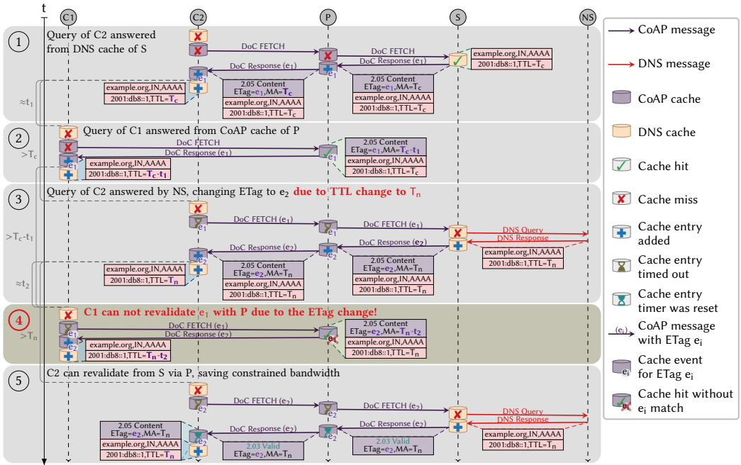
Fig. 3. A name resolution using the DoH-like caching scheme in DoC. DoC clients C1 and C2 query AAAA records for example.org from a DoC server S via a DoC-agnostic CoAP proxy P (1) (2). Only when a DNS cache miss at S occurs, the DNS name server NS is queried (3). A cache hit at P for a query from C2 adapts the TTL, causing cache re-validation to fail and to resend all information (4). Only C1 can leverage cache validation immediately just after the Max-Age (MA) update (5).
