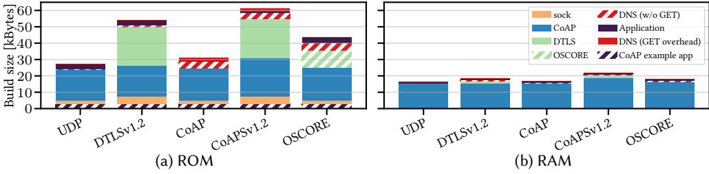
Fig. 5. Memory consumption of each DNS transport with existing CoAP example application.
