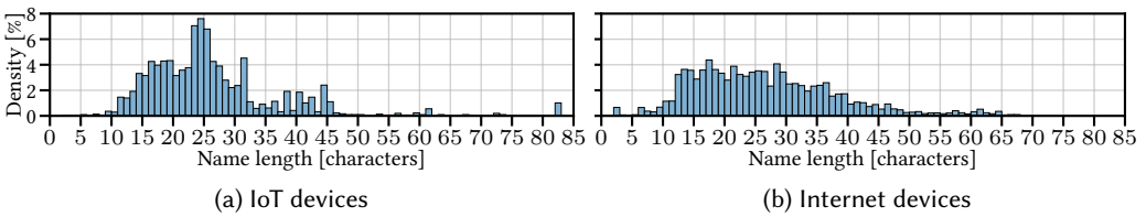
Fig. 1. Distribution of name lengths; names queried by different devices connected via the Internet.
