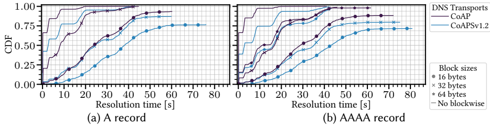
Fig. 15. Resolution times for 50 queries using FETCH with block-wise transfer. Block size 64 was only used with AAAA records, as DNS responses for A record stay below 64 bytes in size.
