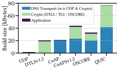
Fig. 8. Code sizes of UDP-based DNS transports.
