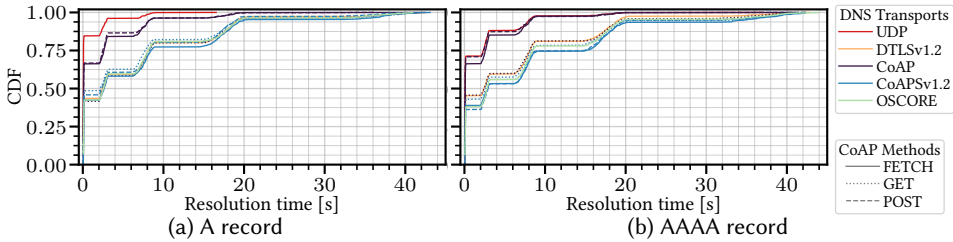
Fig. 7. Resolution times for 50 queries (Poisson distributed with \lambda = 5 queries/s).
