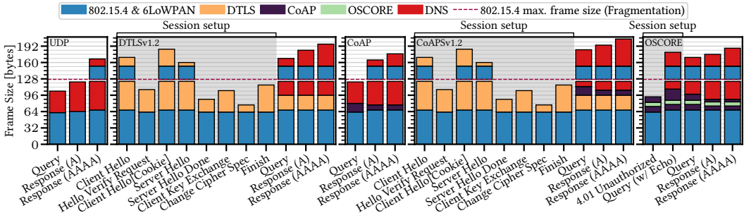
Fig. 6. Maximum link layer packet sizes for each transport when resolving a name with a length of 24 characters for a single record (A or AAAA respectively).
