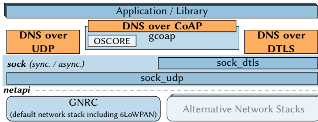
Fig. 13. DNS, DoDTLS, and DoC in RIOT.
