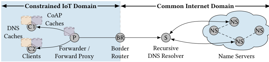
Fig. 2. Typical deployment of the DNS over CoAP (DoC) architecture. DoC protects name resolution between the clients running on IoT devices and the recursive DNS resolver.
